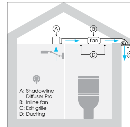
Ceiling installation
